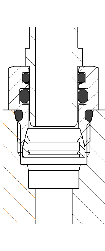
Fig. 23: Schematic diagram for a male gauge
