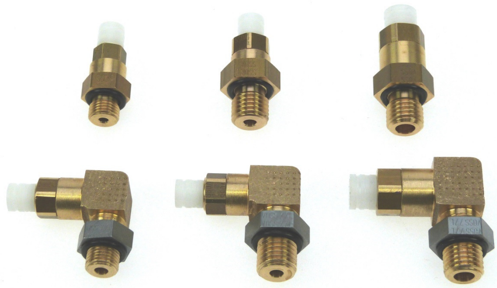
Fig. 9: Socket variants of VOSS quick connect system 203 (examples)
