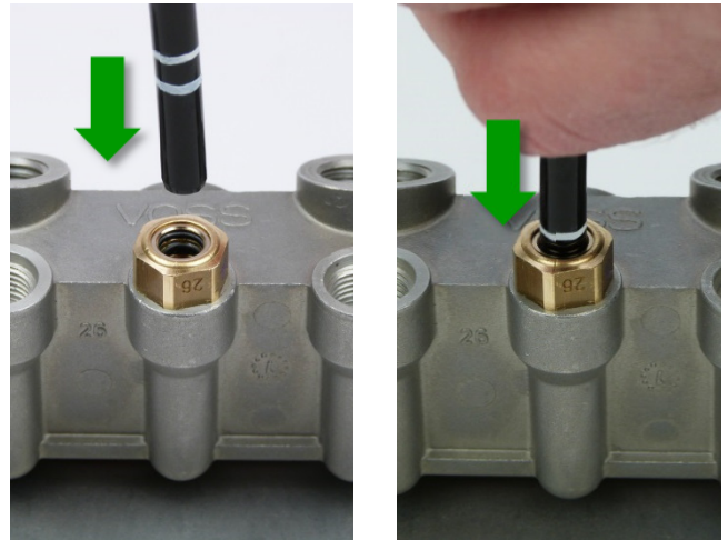
Figs. 19+20: Pushing-in the polyamide tube
