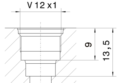
Fig. 8: Profiled bore for V 12 x 1 thread
