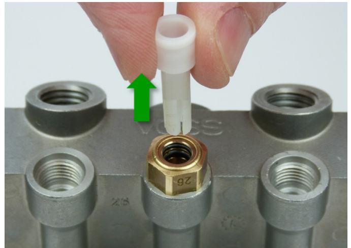
Fig. 16: Pulling out the assembly plug
