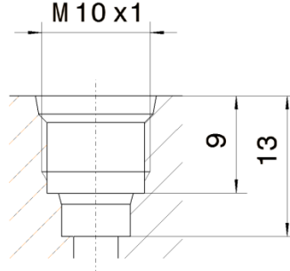
Fig. 4: Profiled bore for M 10 x 1 thread
