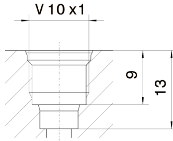
Fig. 7: Profiled bore for V 10 x 1 thread
