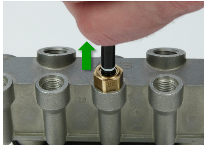
Fig. 23: Pulling back the polyamide tube
