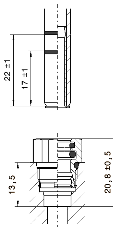
Fig. 22: Push-in depths and dimensions NS 8
