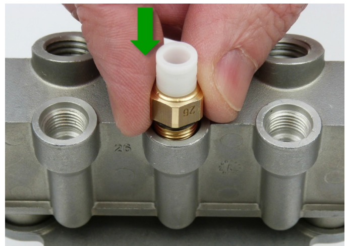
Fig. 12: Positioning the assy at right angles
