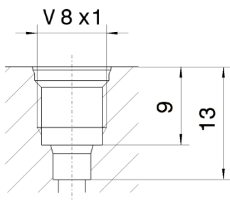
Fig. 6: Profiled bore for V 8 x 1 thread
