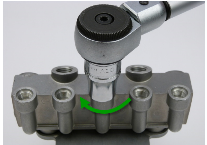
Fig. 14: Tightening with a torque wrench
