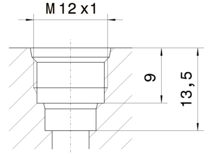
Fig. 5: Profiled bore for M 12 x 1 thread
