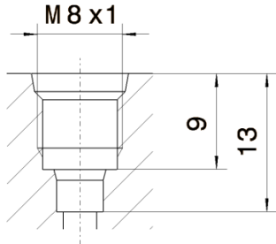
Fig. 3: Profiled bore for M 8 x 1 thread
