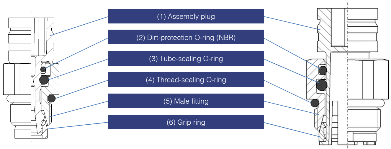
Fig. 1: Components of the assy VOSS quick connect system 203 (left: NS 4, right: NS 8)
