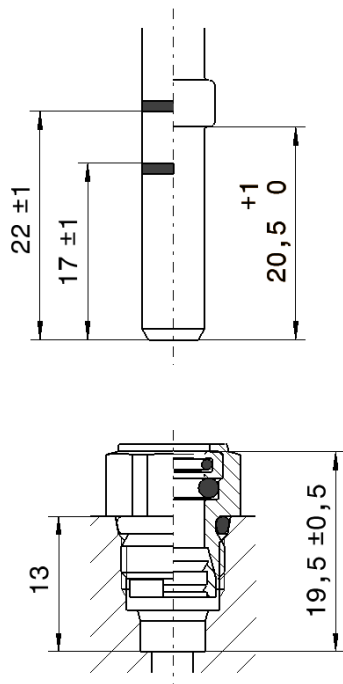
Fig. 21: Push-in depths and dimensions NS 4 and NS 6
